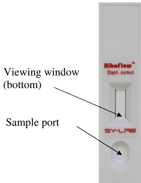
Fig. 1: RiboFlow Staphylococcus aureus lateral flow assay device
